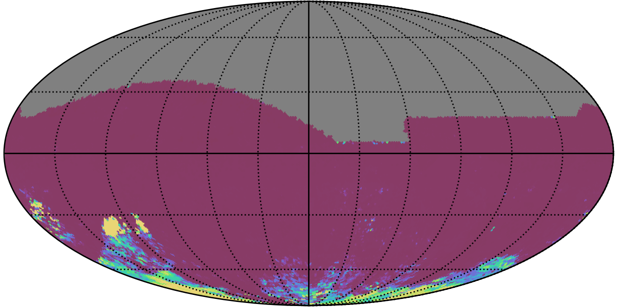
early_ss_template_fpextra2.0_v3.4_10yrs All sky ri bands: 75th Percentile Intranight Timespan
