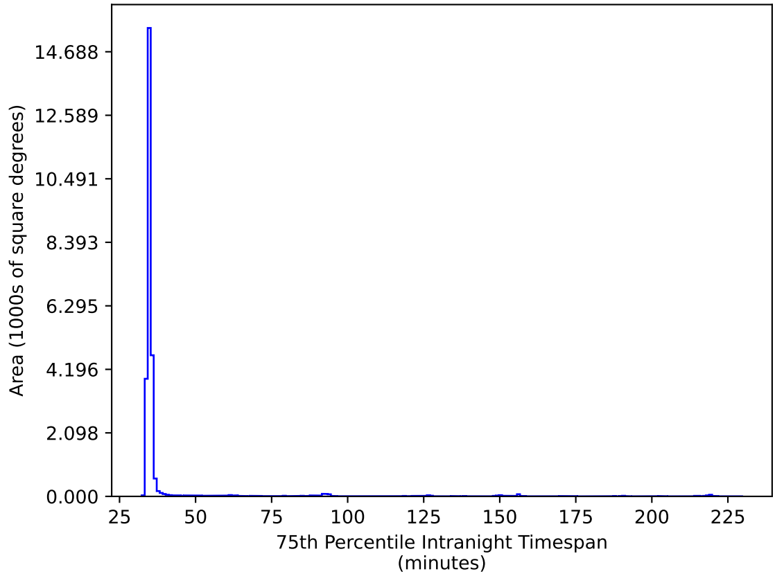
early_ss_template_fpextra2.0_v3.4_10yrs All sky ri bands: 75th Percentile Intranight Timespan
