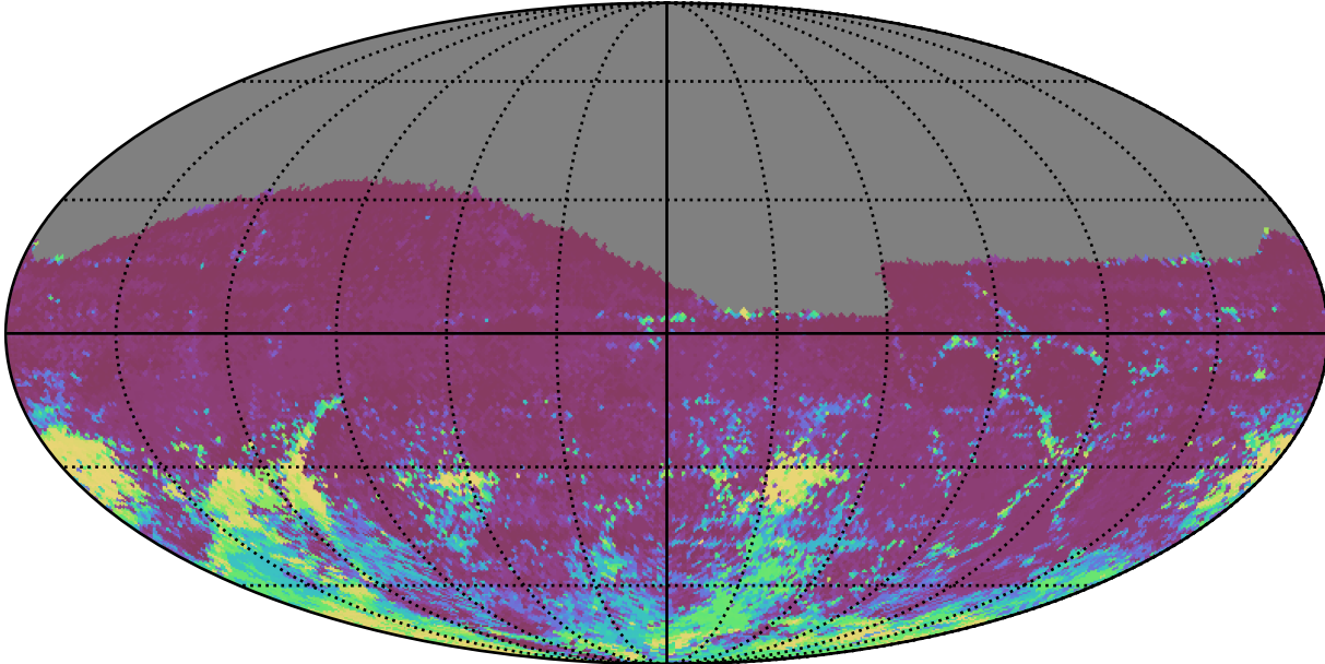
early_ss_template_fpextra2.0_v3.4_10yrs All sky r band: 75th Percentile Intranight Timespan
