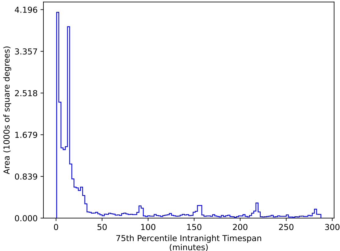
early_ss_template_fpextra2.0_v3.4_10yrs All sky r band: 75th Percentile Intranight Timespan
