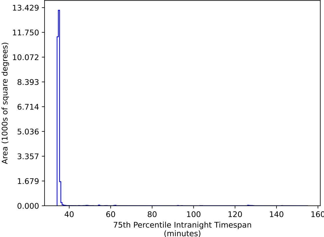
early_ss_template_fpextra2.0_v3.4_10yrs All sky iz bands: 75th Percentile Intranight Timespan
