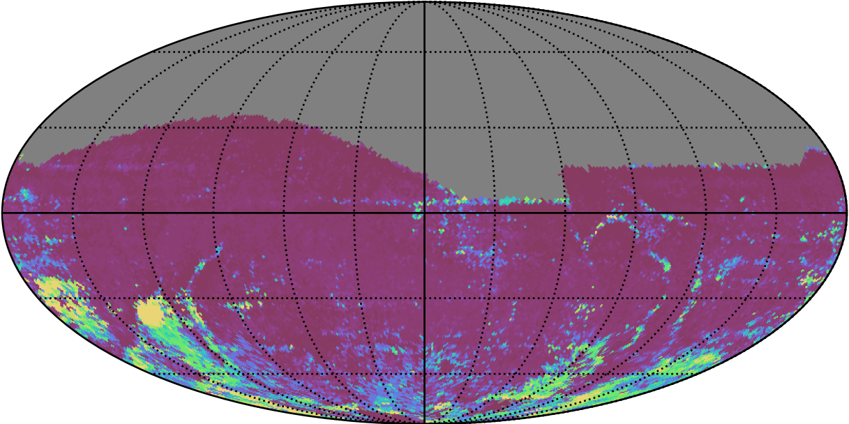
early_ss_template_fpextra2.0_v3.4_10yrs All sky i band: 75th Percentile Intranight Timespan
