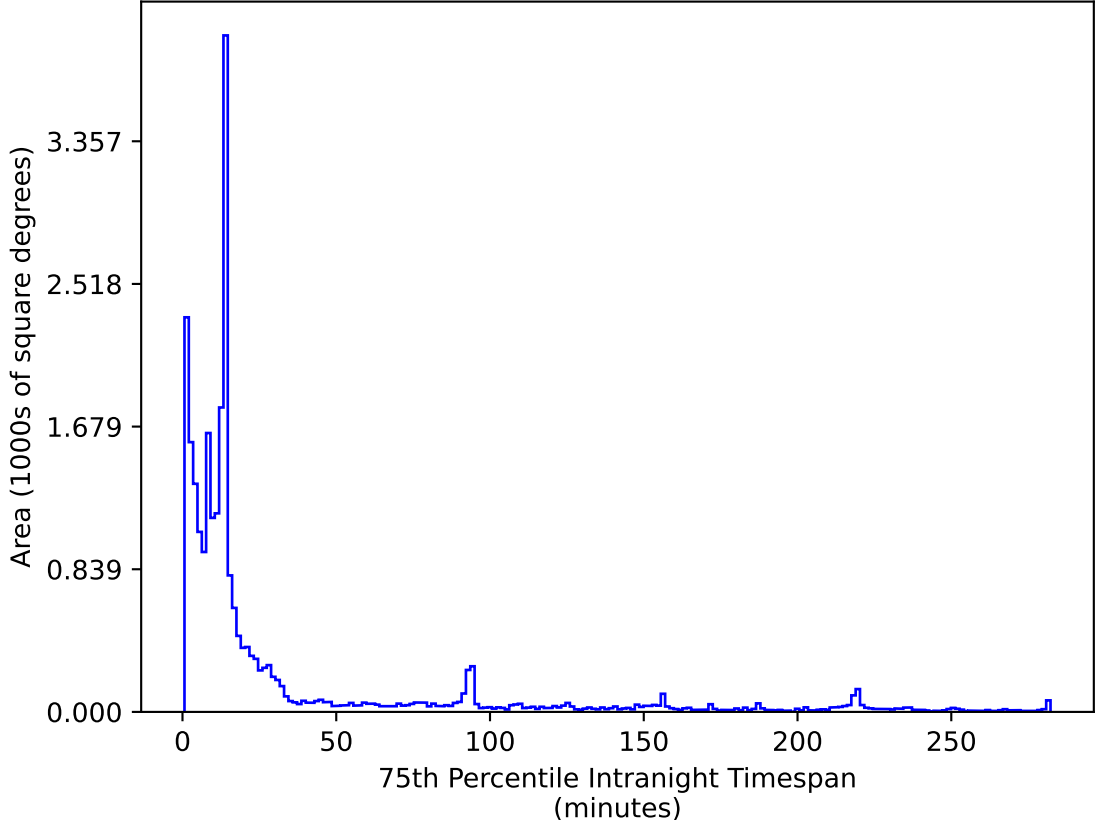
early_ss_template_fpextra2.0_v3.4_10yrs All sky i band: 75th Percentile Intranight Timespan
