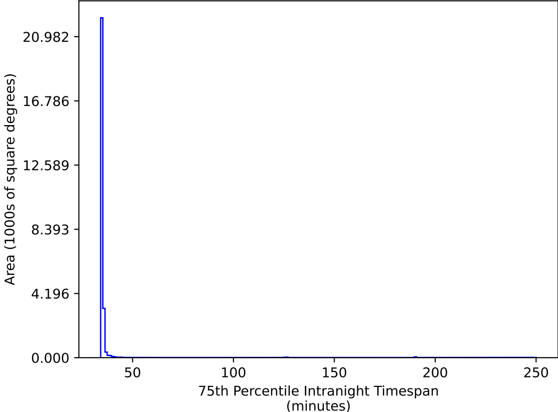
early_ss_template_fpextra2.0_v3.4_10yrs All sky gr bands: 75th Percentile Intranight Timespan
