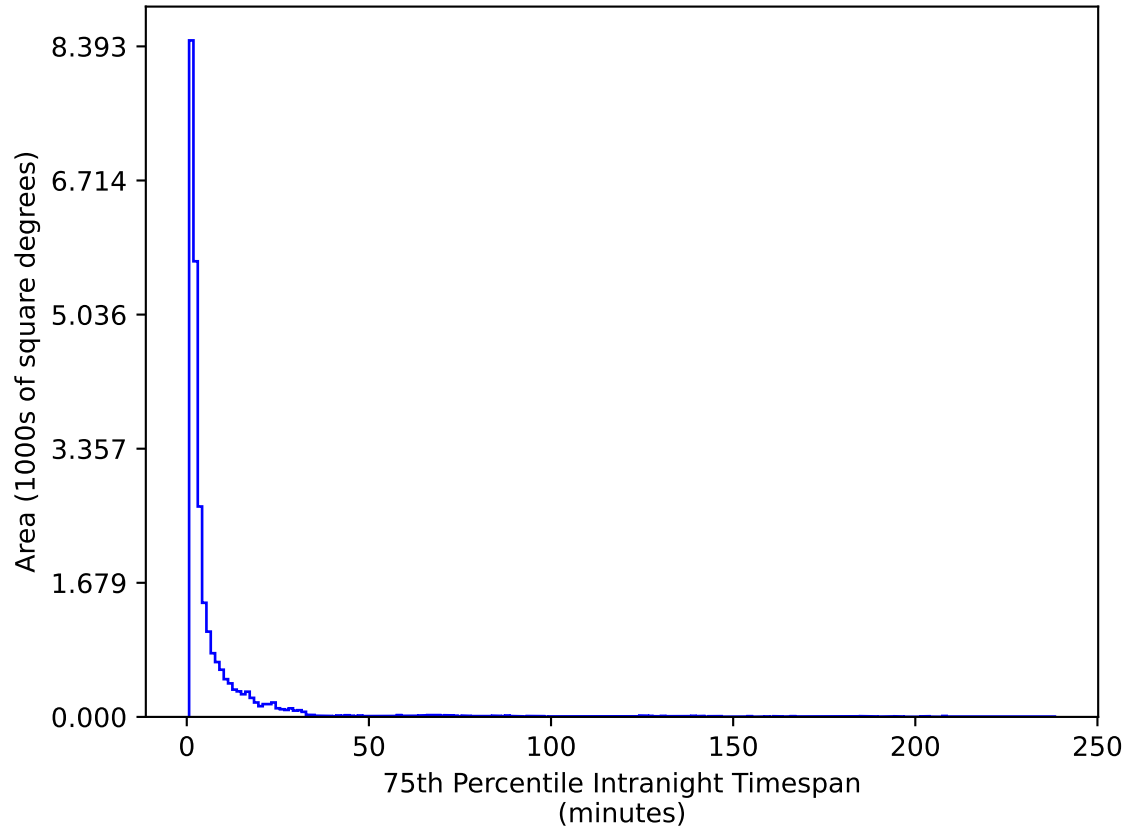
early_ss_template_fpextra2.0_v3.4_10yrs All sky g band: 75th Percentile Intranight Timespan
