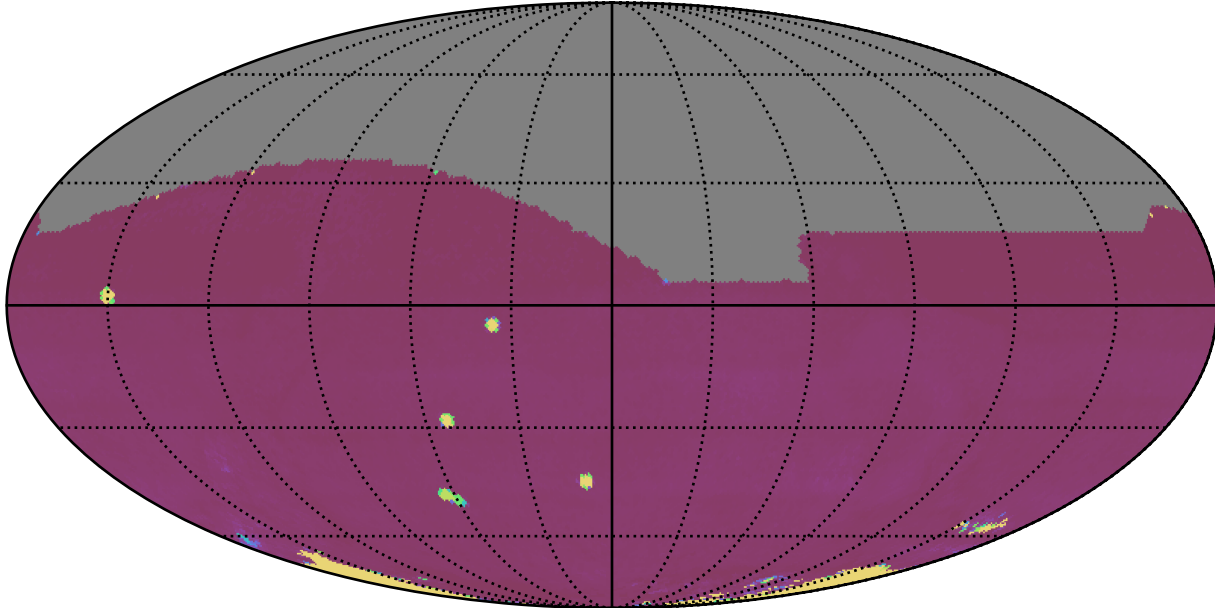
early_ss_template_fpextra2.0_v3.4_10yrs All sky all bands: 75th Percentile Intranight Timespan
