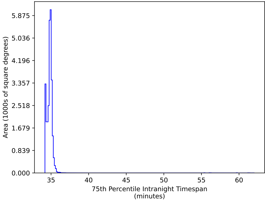
early_ss_template_fpextra2.0_v3.4_10yrs All sky all bands: 75th Percentile Intranight Timespan
