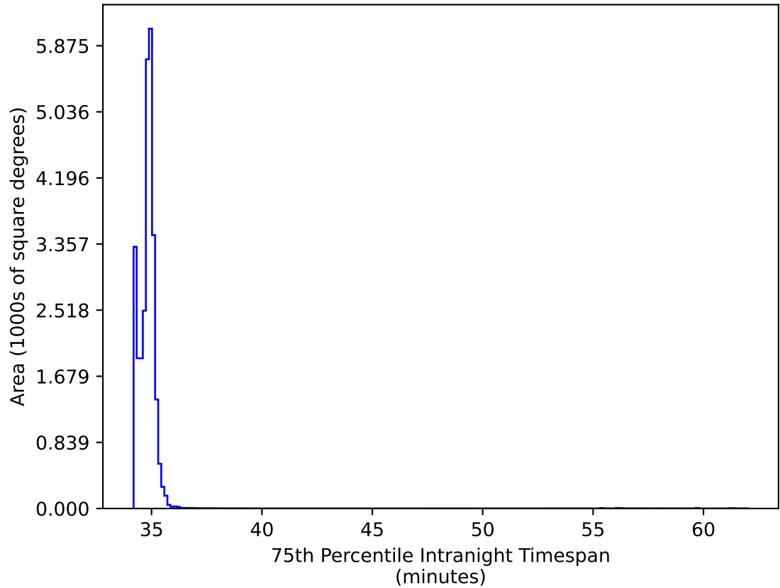
early_ss_template_fpextra2.0_v3.4_10yrs All sky: 75th Percentile Intranight Timespan
