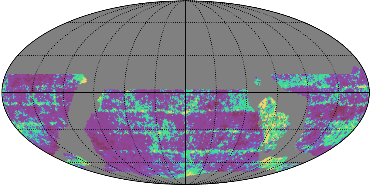
early_ss_template_fpextra2.0_v3.4_10yrs WFD z band: 20thPercentile Inter-Night Gap
