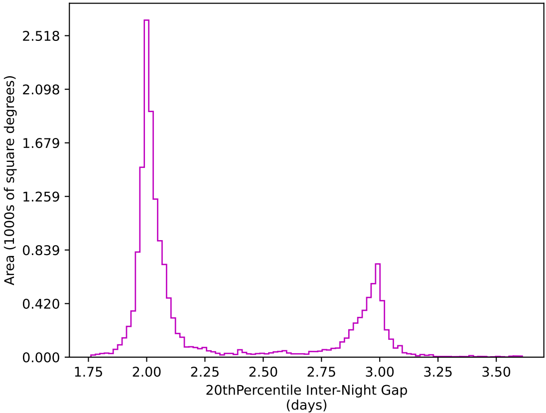
early_ss_template_fpextra2.0_v3.4_10yrs WFD z band: 20thPercentile Inter-Night Gap
