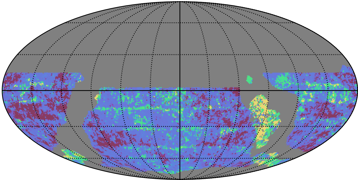
early_ss_template_fpextra2.0_v3.4_10yrs WFD y band: 20thPercentile Inter-Night Gap
