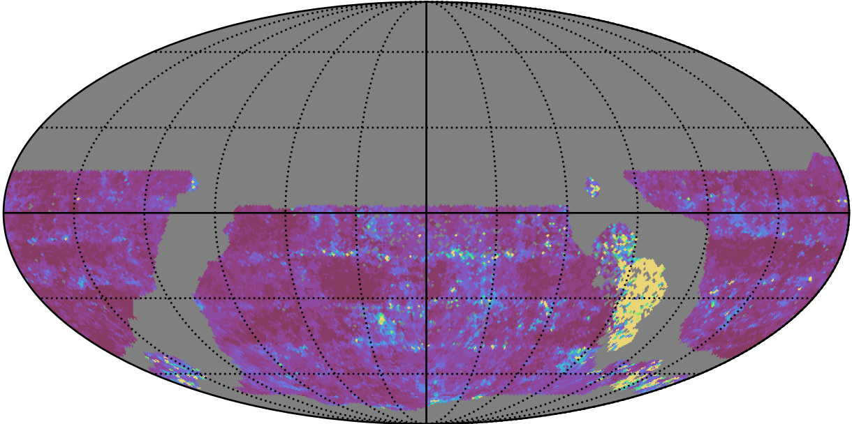
early_ss_template_fpextra2.0_v3.4_10yrs WFD u band: 20thPercentile Inter-Night Gap
