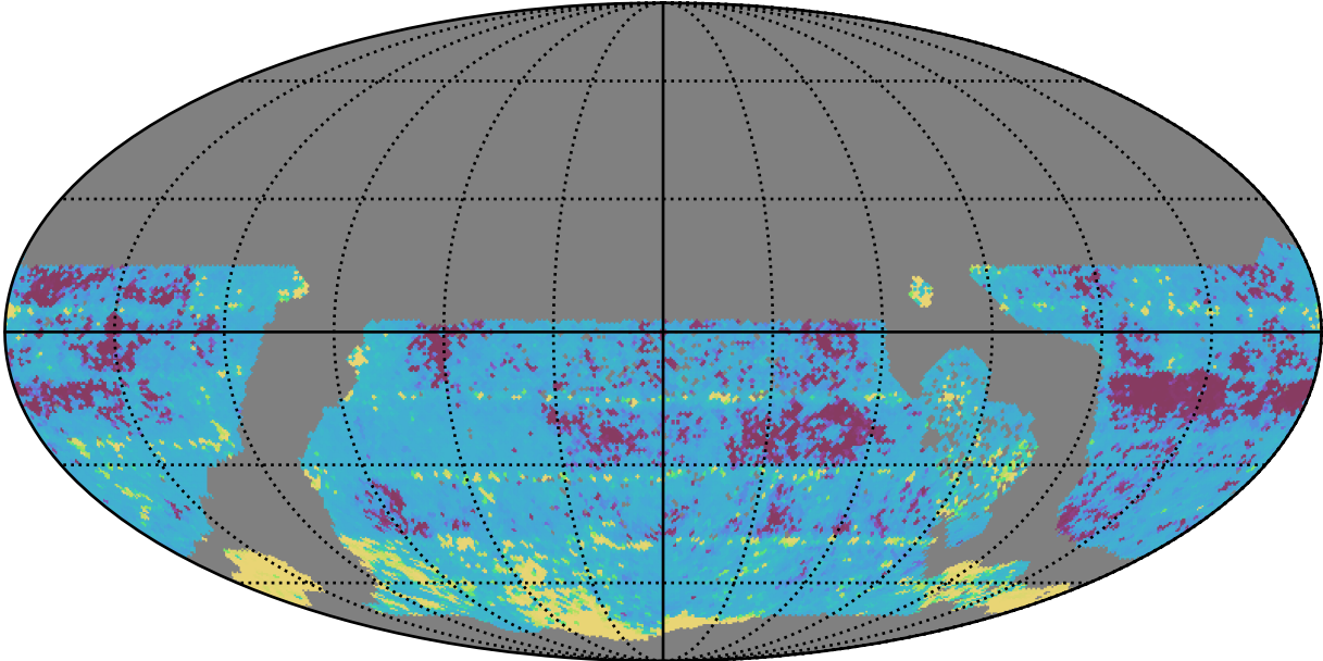
early_ss_template_fpextra2.0_v3.4_10yrs WFD r band: 20thPercentile Inter-Night Gap
