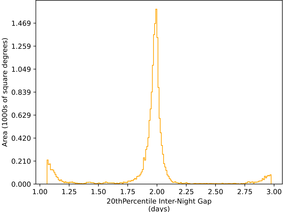
early_ss_template_fpextra2.0_v3.4_10yrs WFD r band: 20thPercentile Inter-Night Gap
