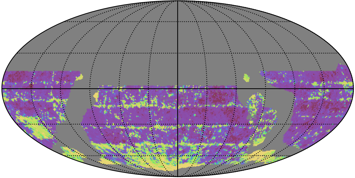
early_ss_template_fpextra2.0_v3.4_10yrs WFD i band: 20thPercentile Inter-Night Gap
