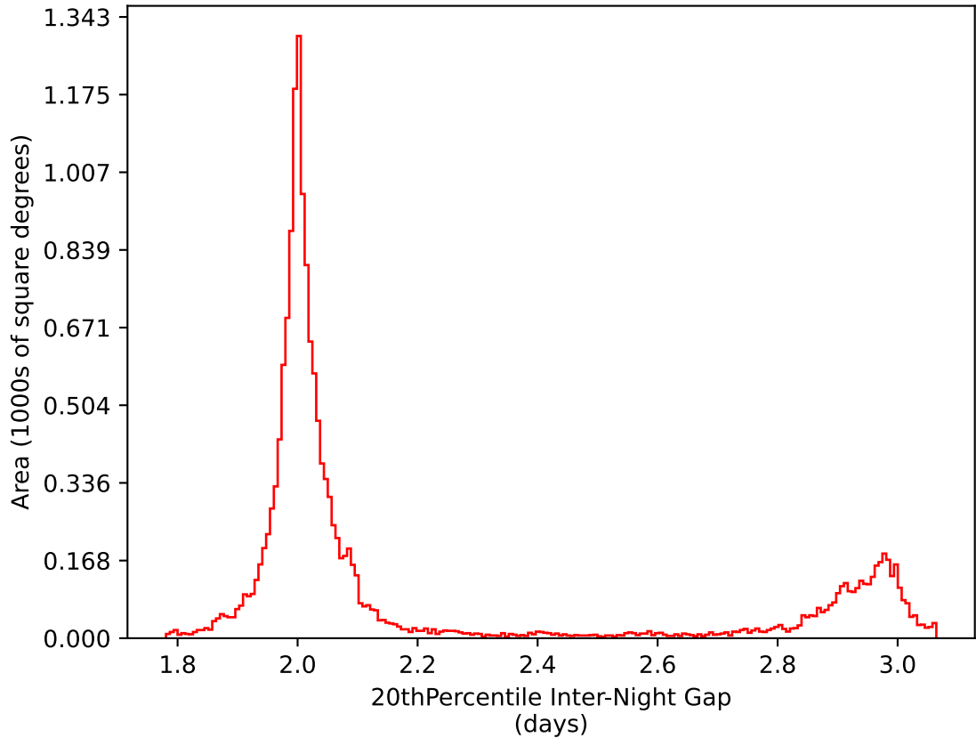
early_ss_template_fpextra2.0_v3.4_10yrs WFD i band: 20thPercentile Inter-Night Gap
