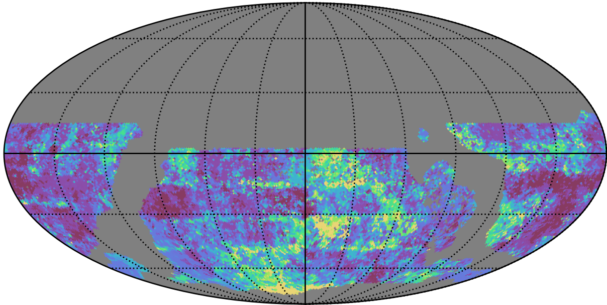
early_ss_template_fpextra2.0_v3.4_10yrs WFD g band: 20thPercentile Inter-Night Gap
