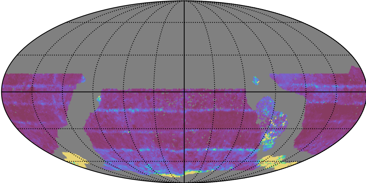
early_ss_template_fpextra2.0_v3.4_10yrs WFD all bands: 20thPercentile Inter-Night Gap
