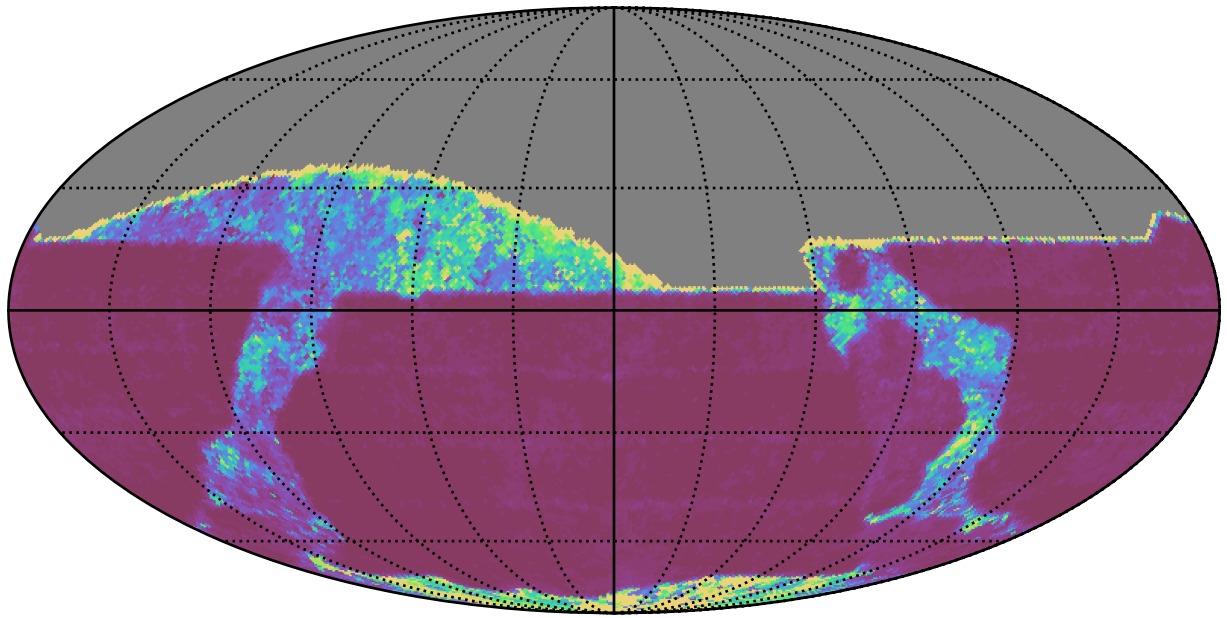
early_ss_template_fpextra2.0_v3.4_10yrs All sky z band: 20thPercentile Inter-Night Gap
