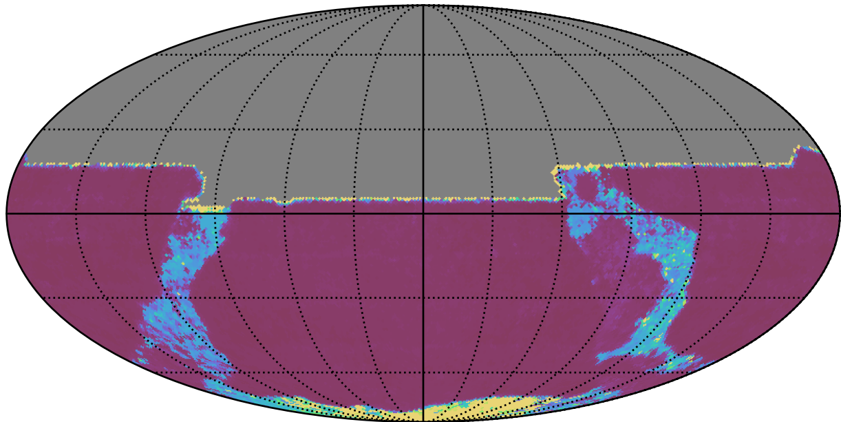
early_ss_template_fpextra2.0_v3.4_10yrs All sky y band: 20thPercentile Inter-Night Gap
