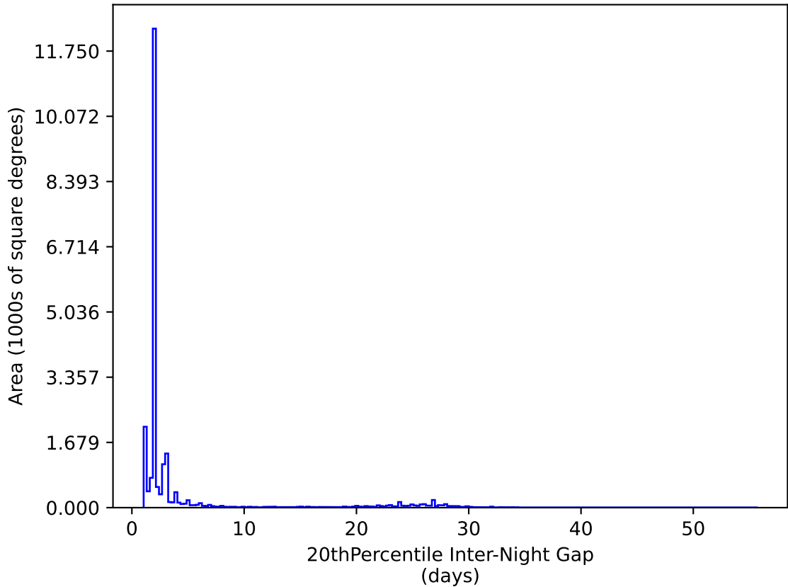
early_ss_template_fpextra2.0_v3.4_10yrs All sky y band: 20thPercentile Inter-Night Gap
