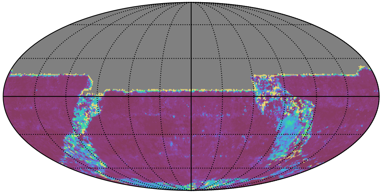
early_ss_template_fpextra2.0_v3.4_10yrs All sky u band: 20thPercentile Inter-Night Gap
