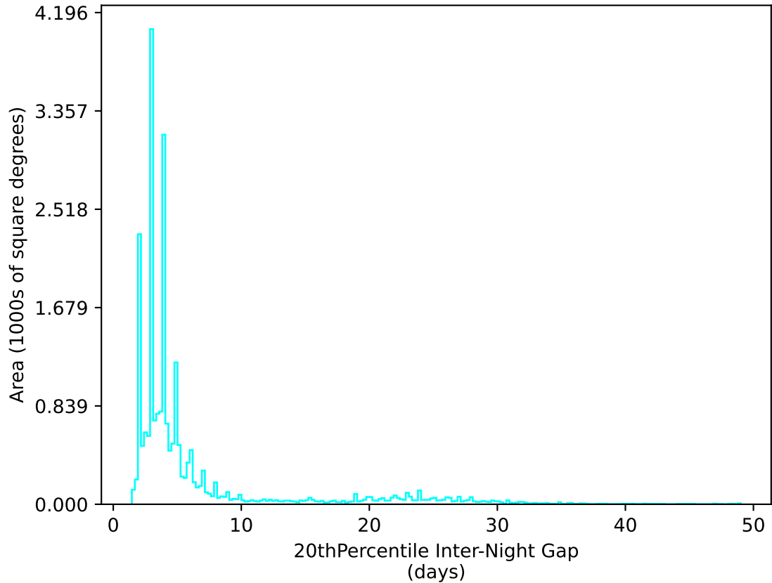
early_ss_template_fpextra2.0_v3.4_10yrs All sky u band: 20thPercentile Inter-Night Gap
