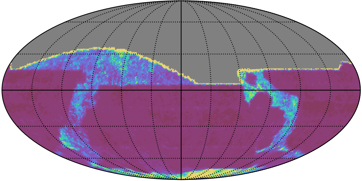
early_ss_template_fpextra2.0_v3.4_10yrs All sky r band: 20thPercentile Inter-Night Gap
