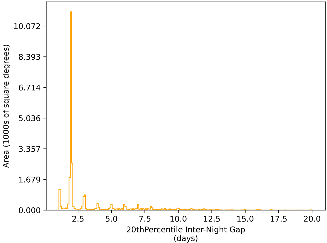
early_ss_template_fpextra2.0_v3.4_10yrs All sky r band: 20thPercentile Inter-Night Gap
