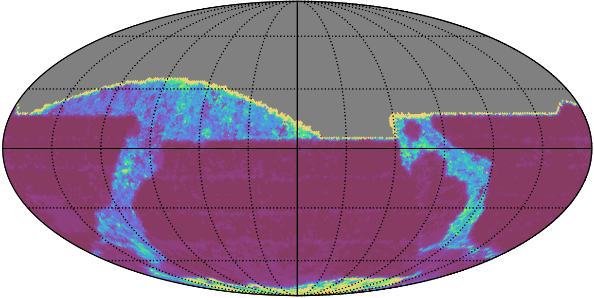
early_ss_template_fpextra2.0_v3.4_10yrs All sky i band: 20thPercentile Inter-Night Gap
