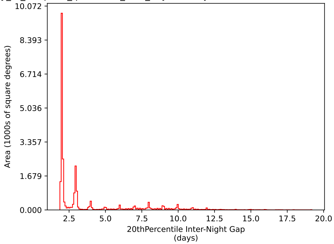
early_ss_template_fpextra2.0_v3.4_10yrs All sky i band: 20thPercentile Inter-Night Gap
