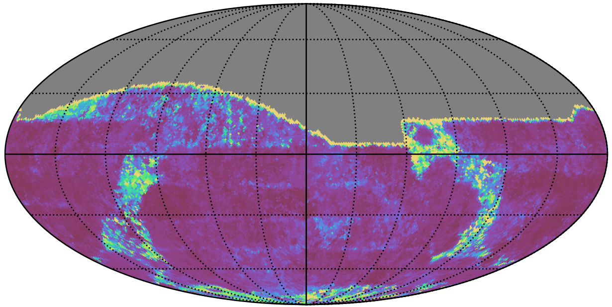
early_ss_template_fpextra2.0_v3.4_10yrs All sky g band: 20thPercentile Inter-Night Gap
