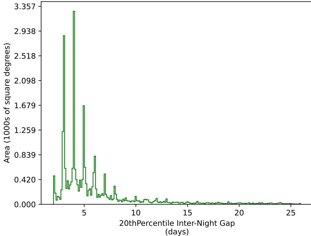
early_ss_template_fpextra2.0_v3.4_10yrs All sky g band: 20thPercentile Inter-Night Gap
