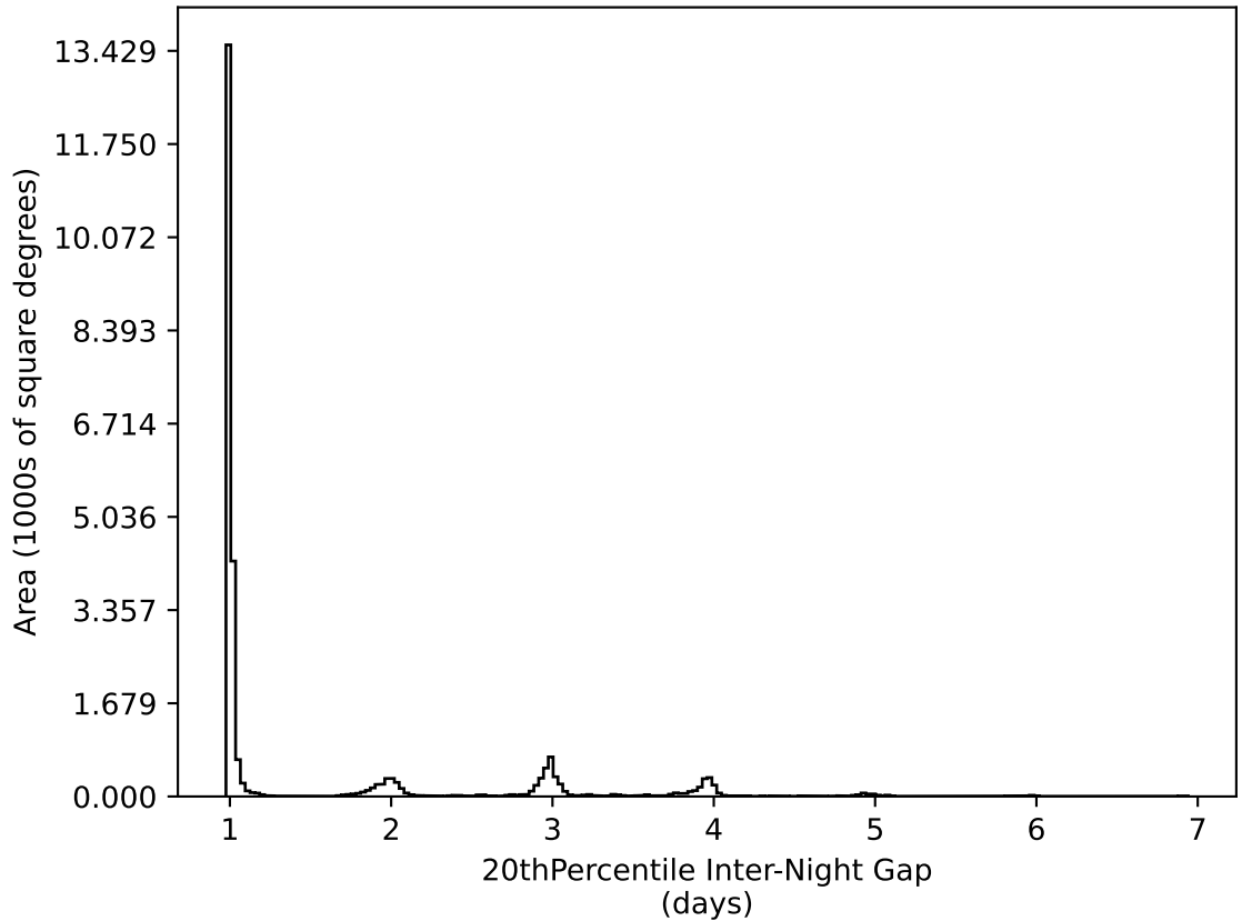
early_ss_template_fpextra2.0_v3.4_10yrs All sky all bands: 20thPercentile Inter-Night Gap
