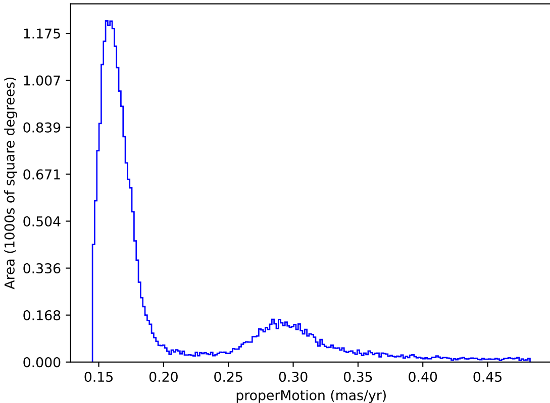
early_ss_template_fpextra2.0_v3.4_10yrs : properMotion
