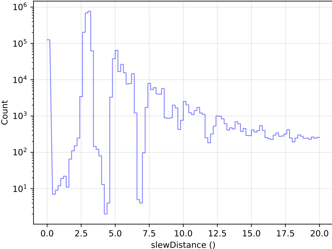
early_ss_template_fpextra2.0_v3.4_10yrs All visits: Zoom Slew Distance Histogram
