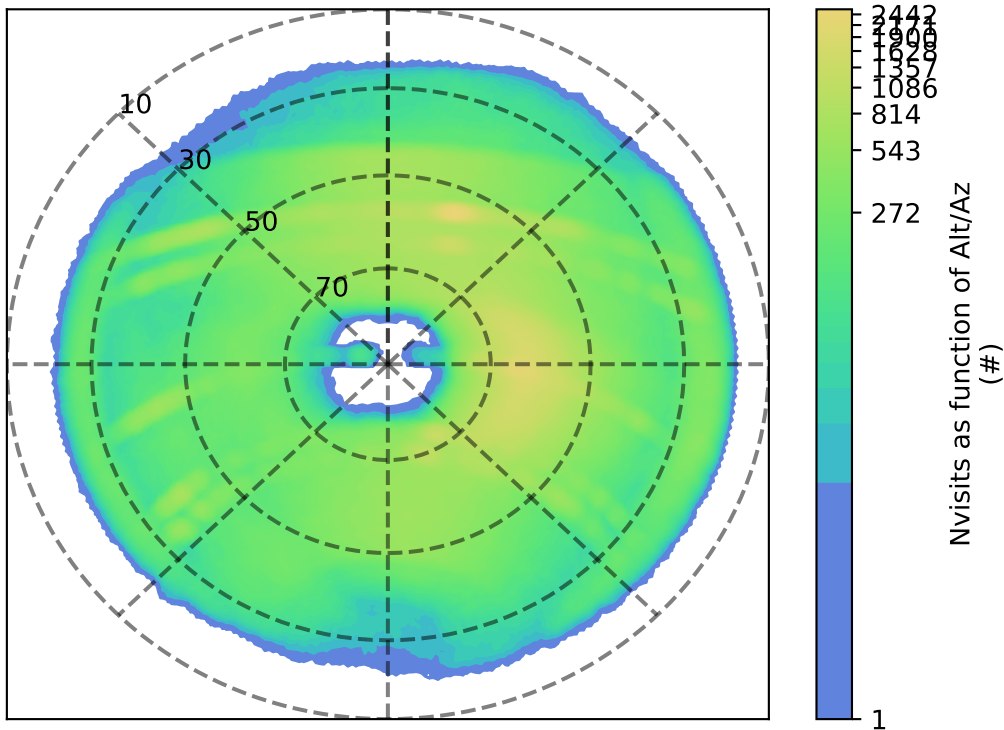
early_ss_template_fpextra2.0_v3.4_10yrs z: Nvisits as function of Alt/Az
