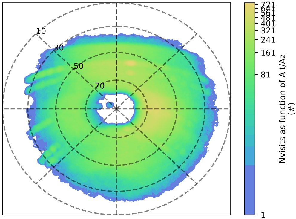
early_ss_template_fpextra2.0_v3.4_10yrs u: Nvisits as function of Alt/Az
