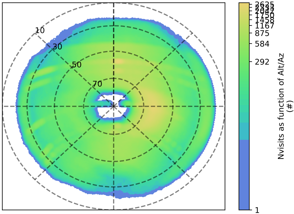
early_ss_template_fpextra2.0_v3.4_10yrs i: Nvisits as function of Alt/Az
