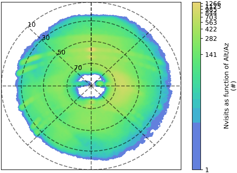
early_ss_template_fpextra2.0_v3.4_10yrs g: Nvisits as function of Alt/Az
