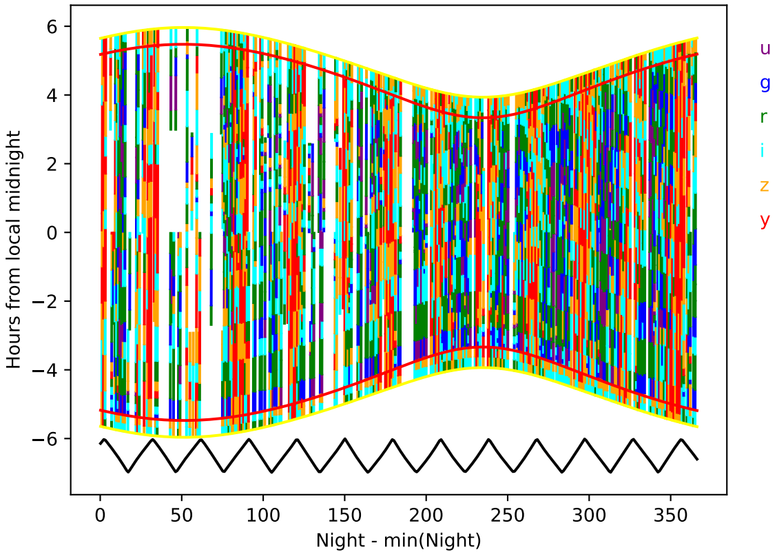
early_ss_template_fpextra2.0_v3.4_10yrs year 9-10: Hourglass
