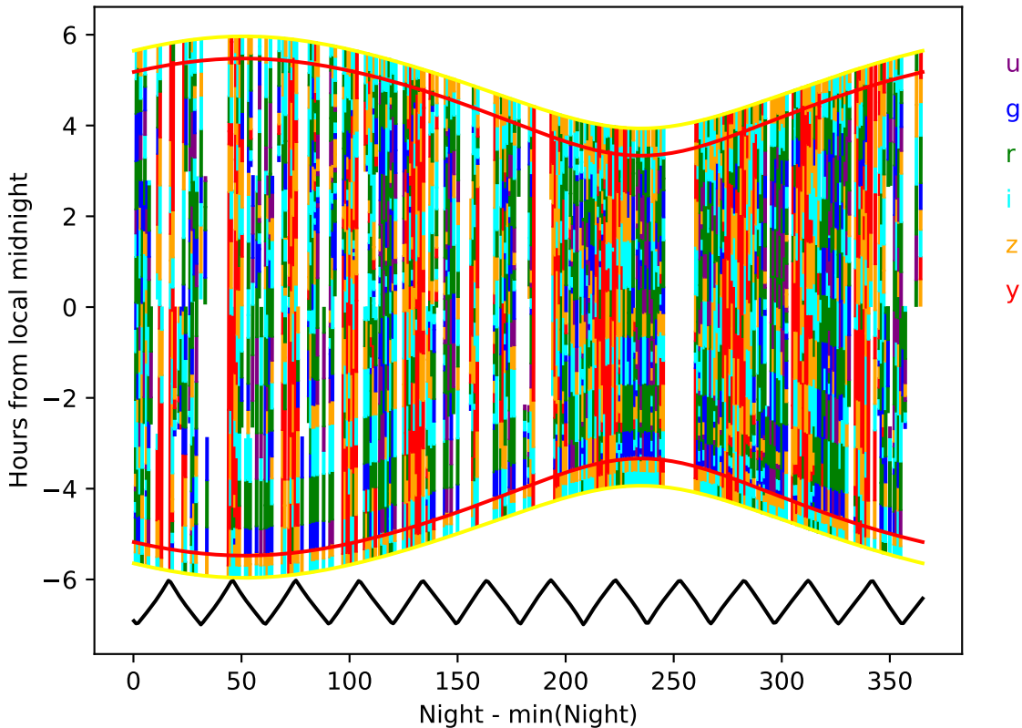
early_ss_template_fpextra2.0_v3.4_10yrs year 5-6: Hourglass
