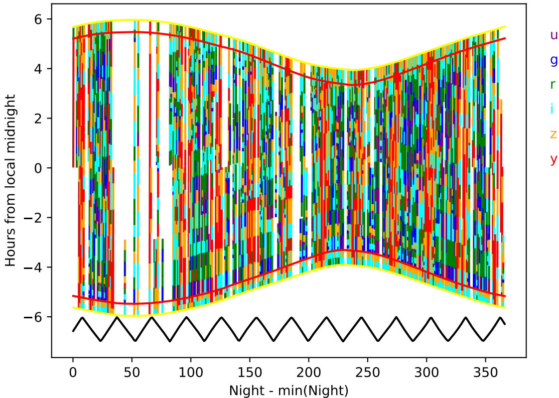
early_ss_template_fpextra2.0_v3.4_10yrs year 3-4: Hourglass
