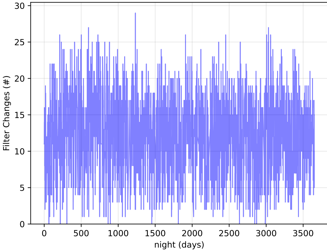
early_ss_template_fpextra2.0_v3.4_10yrs : Filter Changes
