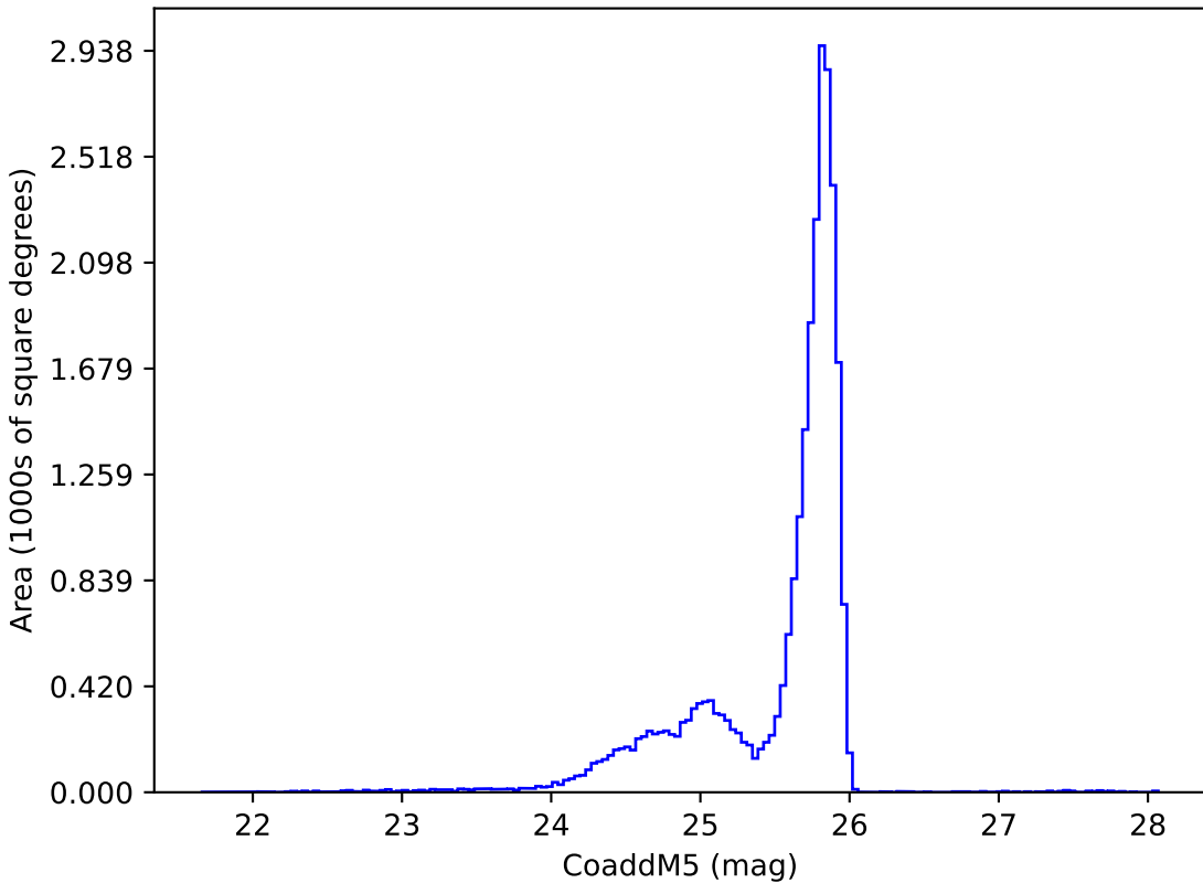
early_ss_template_fpextra2.0_v3.4_10yrs z: CoaddM5
