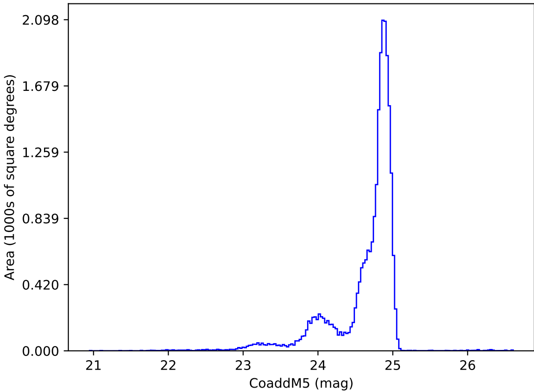
early_ss_template_fpextra2.0_v3.4_10yrs y: CoaddM5
