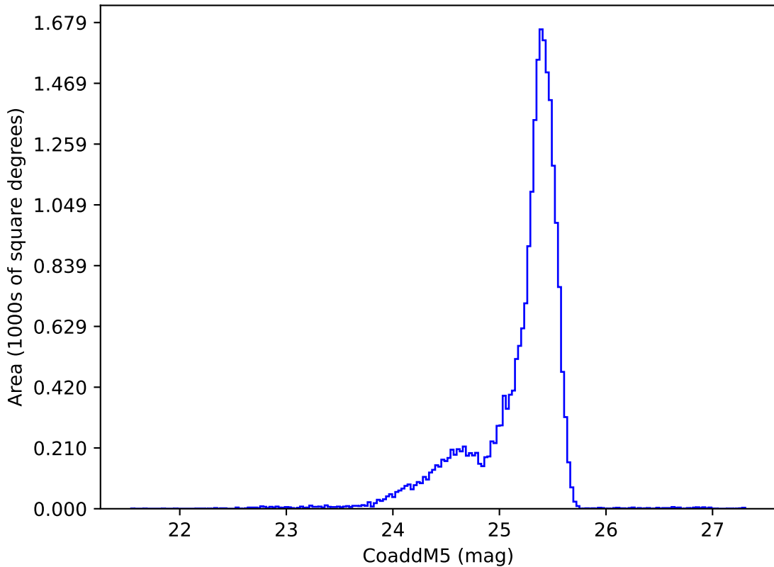
early_ss_template_fpextra2.0_v3.4_10yrs u: CoaddM5
