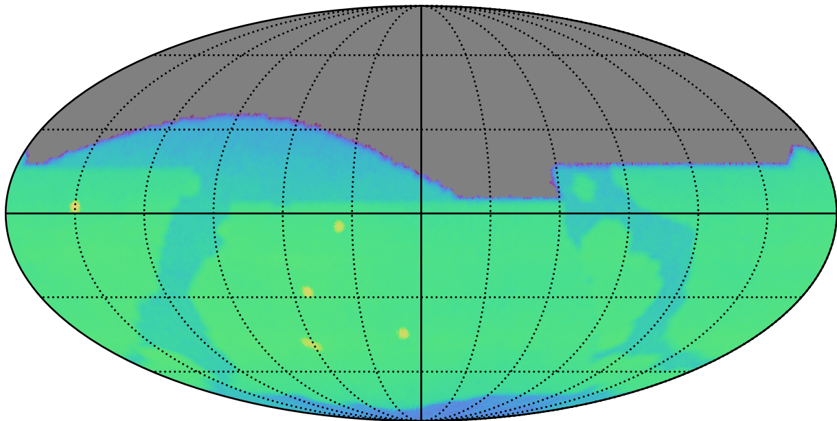
early_ss_template_fpextra2.0_v3.4_10yrs r: CoaddM5
