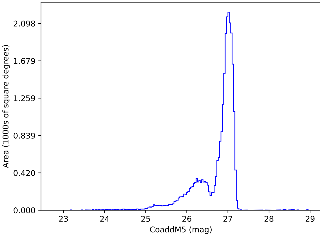
early_ss_template_fpextra2.0_v3.4_10yrs r: CoaddM5
