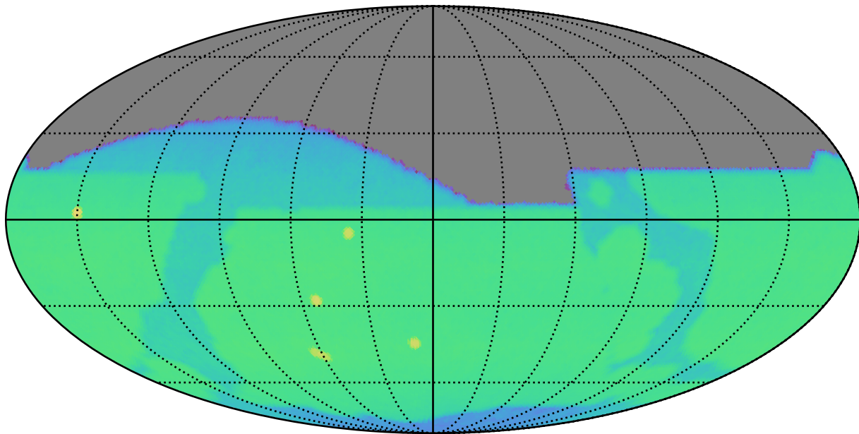
early_ss_template_fpextra2.0_v3.4_10yrs i: CoaddM5
